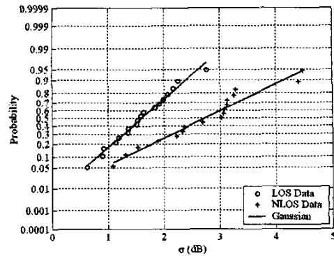
Figure 4: CDF of standard deviation of shadow fading.
