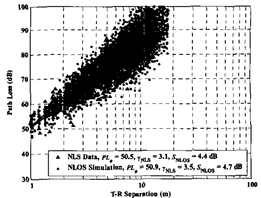
Figure 6: Simulation vs. measured NLOS path loss.
