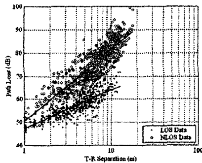
Figure 2: Path loss vs. T-R separation.
