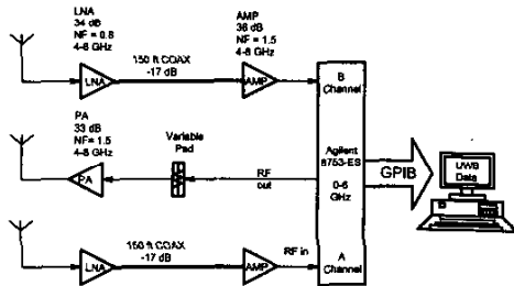
Figure 1: Channel sounder configuration.
