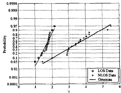
Figure 5: CDF of path loss exponent.
